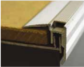
WITH BASE PROFILE "TRIO GRIP"
